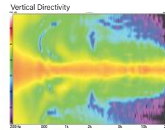
Vertical Directivity
